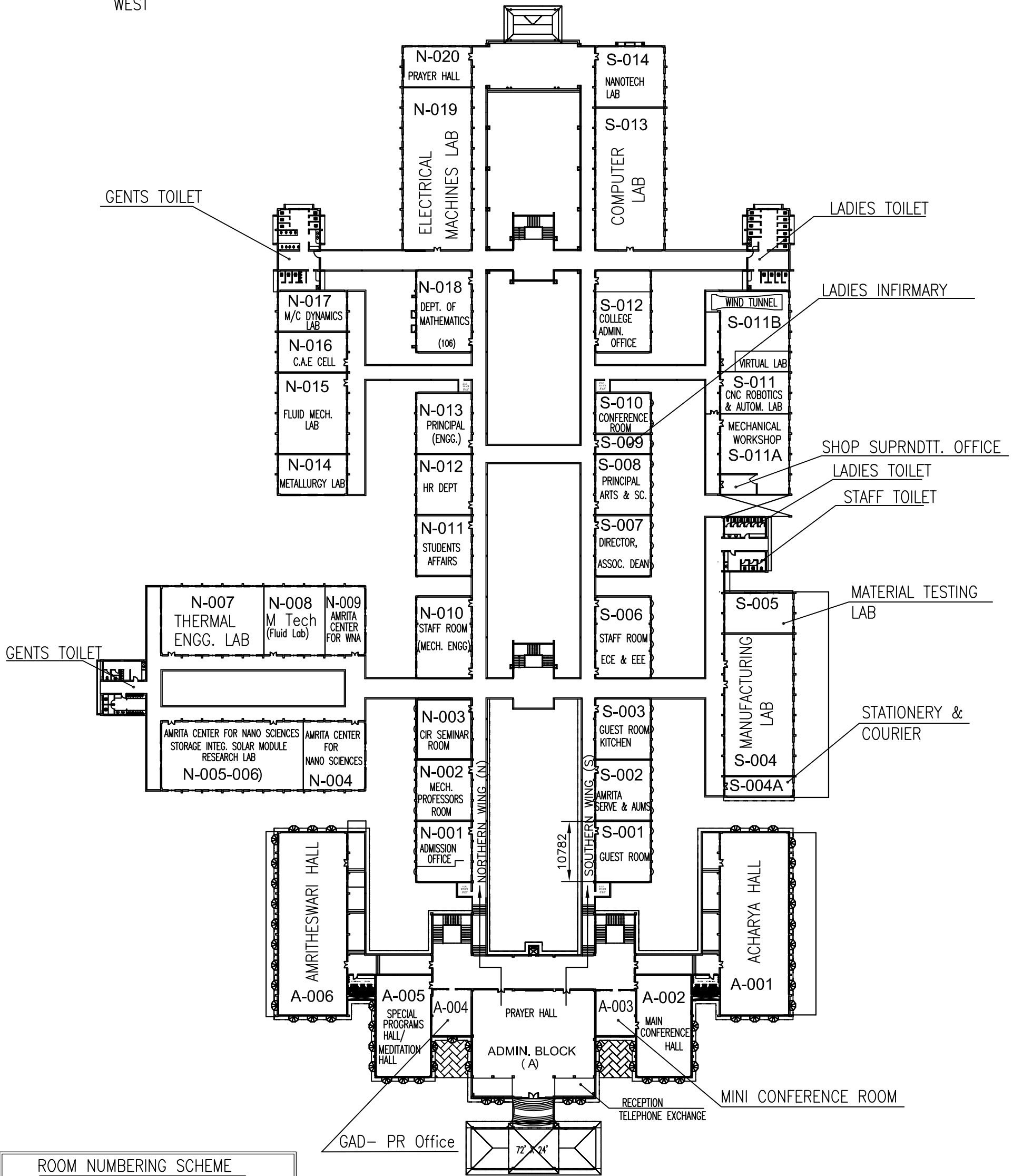
GROUND FLOOR PLAN (ROOM NOS START WITH 0)
