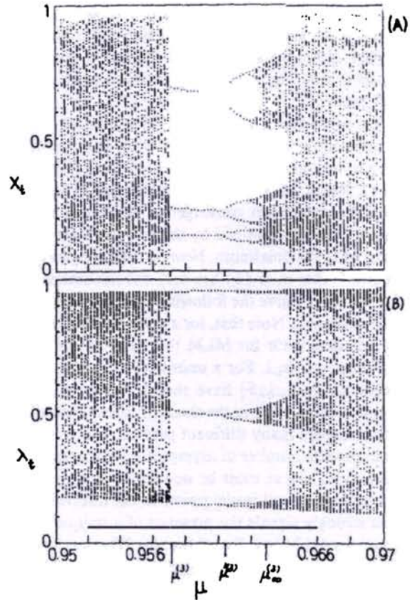
Fig. 2. Bifurcation structure of MLM for the parameter range 0.95 < \mu < 0.97 projected (A) onto the (X_t, \mu) plane and (B) onto the (\lambda_t, \mu) plane.
