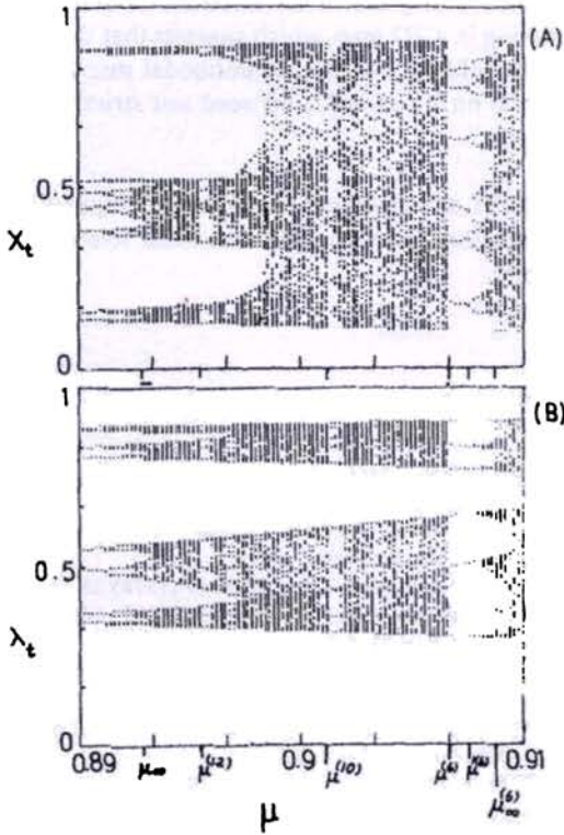
Fig. 1. Bifurcation structure of MLM for the parameter range 0.89 < \mu < 0.91 projected (A) onto the (X_t, \mu) plane and (B) onto the (\lambda_t, \mu) plane which is just the bifurcation structure of the logistic map for the specified range of the parameter.
